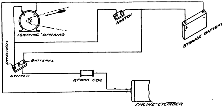
FIG. 229.—Diagram of a Primary Spark Circuit, equipped with a Dynamo and Storage Battery. The dynamo may be used to spark the engine and supply the battery at the same time, or to perform the former function exclusively. The battery is charged when the switch between it and the dynamo is thrown in, if the other switch "dynamo" in the cut. As is obvious from the cut, the dynamo may be cut out altogether, allowing the storage battery to supply current for sparking purposes. When both switches are in, the storage battery will supply current for sparking, until the dynamo has attained its full speed.
